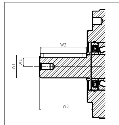
Mounting flange
