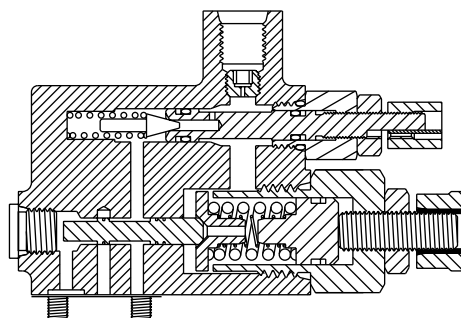
LOAD SENSE OPTION "A" REQ'D W/POWER OPTION "C" OR "HLA" ITEM 93
